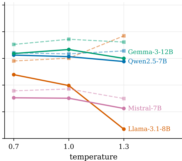
MMLU-Pro
