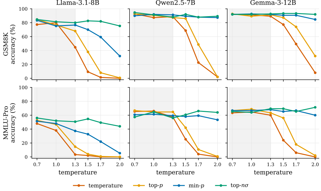
Figure 2: The cliff map. Accuracy versus temperature per sampler (the T \leq 1.0 points come from the main matrix; all at Q8). Every model has a cliff; where it sits is the model property. Truncation shifts the cliff right by tail-cutting strength.
