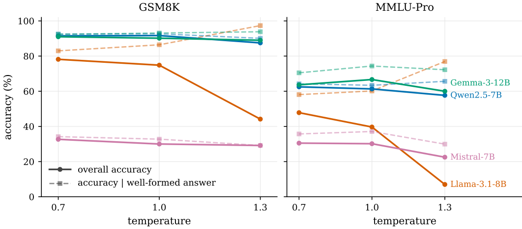
Figure 4: Overall accuracy (solid) versus accuracy among well-formed, strict-parsed answers (dashed) under plain temperature sampling; four models spanning the robustness gradient (the three Qwen3 models are flat and omitted for legibility). The dashed lines stay flat: among well-formed answers, accuracy barely moves with temperature.
