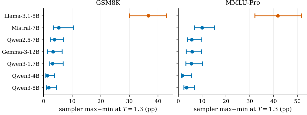
Figure 3: Sampler max-min accuracy spread at T=1.3 per model (95% CIs).
