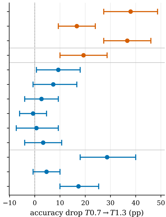
MMLU-Pro
