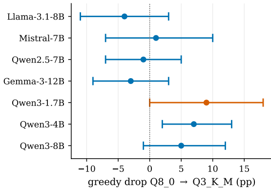
Figure 7: Greedy accuracy drop Q8_0 \rightarrow Q3_K_M per model (95% CIs), pooled tasks.
