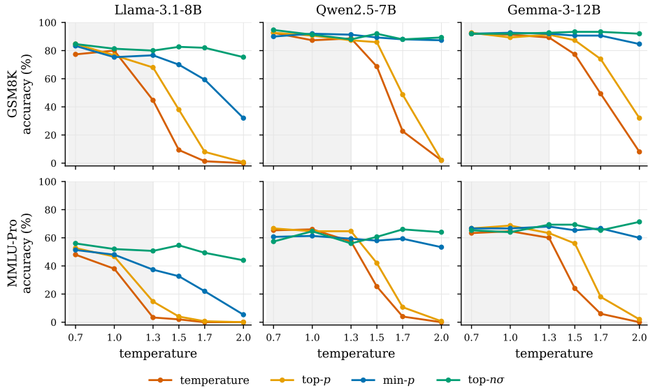
Figure 6: Cliff temperatures (Section 4.4). Accuracy versus temperature per sampler (the T \leq 1.0 points come from the main grid; all at Q8). Each model has a cliff, at a temperature that differs by model. Truncation raises each model’s cliff temperature.
