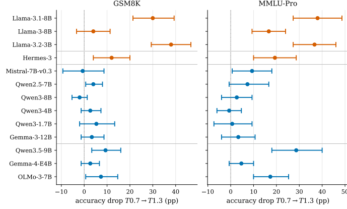
Figure 1: Plain-temperature accuracy drop T_{0.7} \rightarrow T_{1.3} at Q8_0 for the seven grid models, the two additional Llama releases, and the follow-up panel; points with 95% item-clustered bootstrap CIs. Llama-3-based models in orange.
