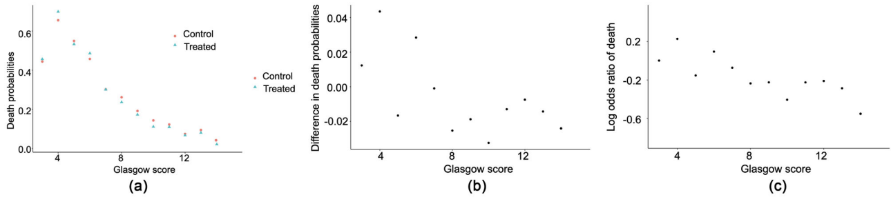
FIGURE 1 Treatment effect of drug Tranexamic acid and Glasgow score. Panel (a) displays the probabilities of death for different Glasgow scores. Panel (b) displays the difference of the treatment and control death probabilities. Panel (c) displays the log-odds ratio of the treatment and control death probabilities.
