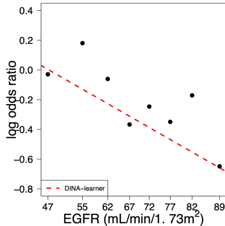
FIGURE 3 EGFR and DINA (log-odds ratio). We divide the participants into eight groups according to their EGFR. We plot the average log-odds ratio of the intervention. We also superimpose the estimated line from the DINA-learner, where we fix the values of the covariates other than EGFR at their averages. Abbreviation: DINA, Difference in NATural parameters. .
