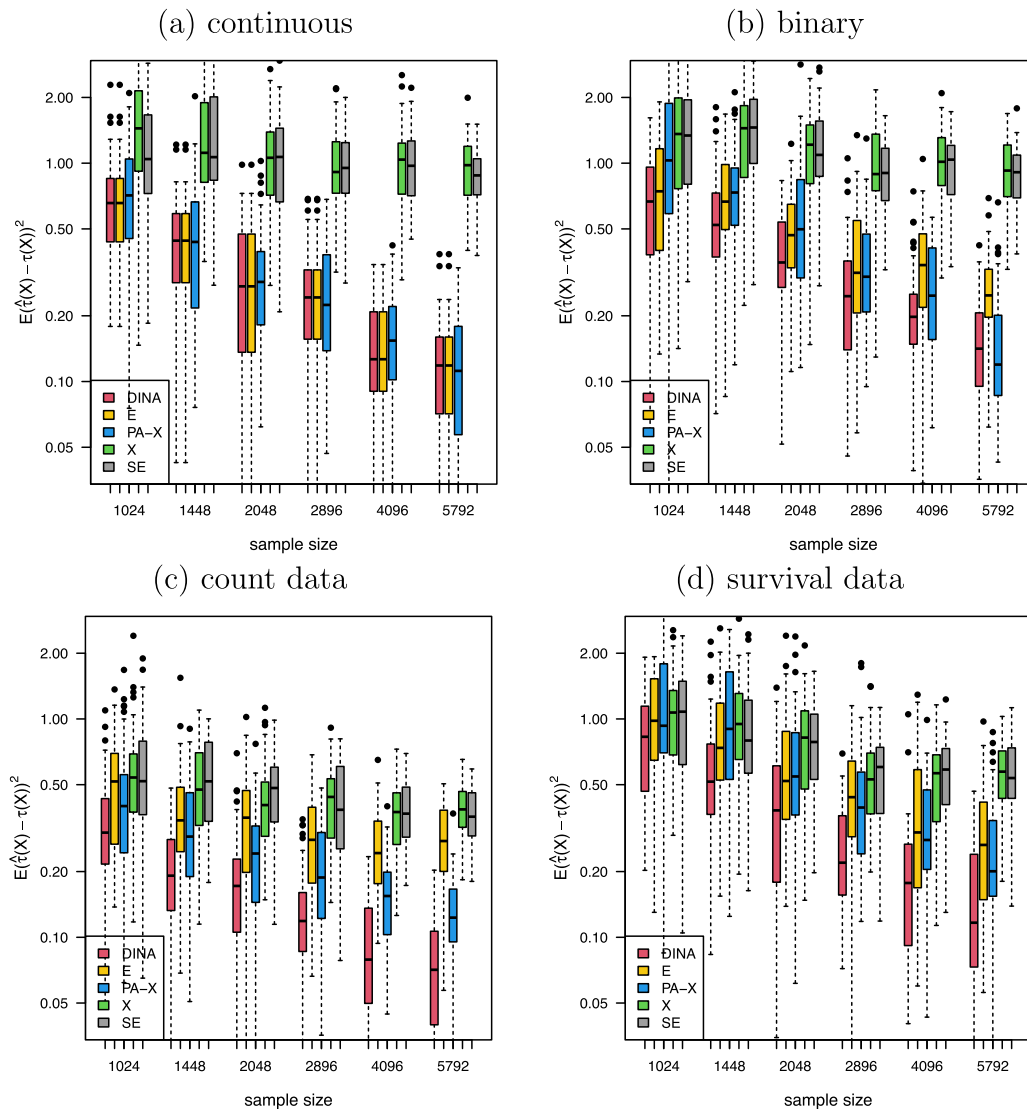
FIGURE 2 Estimation error log-log boxplots. We display the estimation errors \mathbb{E}[(\hat{\tau}(X) - \tau(X))^2] over sample sizes in [1024, 1448, 2048, 2896, 4096, 5792]. We compare five methods: separate estimation (SE), X-learner (X), propensity score adjusted X-learner (PA-X), direct extension of the R-learner (E), and Algorithm 1 (DINA). We adopt the response model (19) and consider four types of responses: (a) continuous (Gaussian), (b) binary (Bernoulli), (c) count data (Poisson), (d) survival data (Cox model with uniform censoring, 75% units censored). We estimate the propensity score by logistic regression, and estimate the natural parameters by fitting generalized linear models or maximizing Cox partial likelihoods. We repeat all experiments 100 times. Abbreviation: DINA, Difference in Natural parameters.
