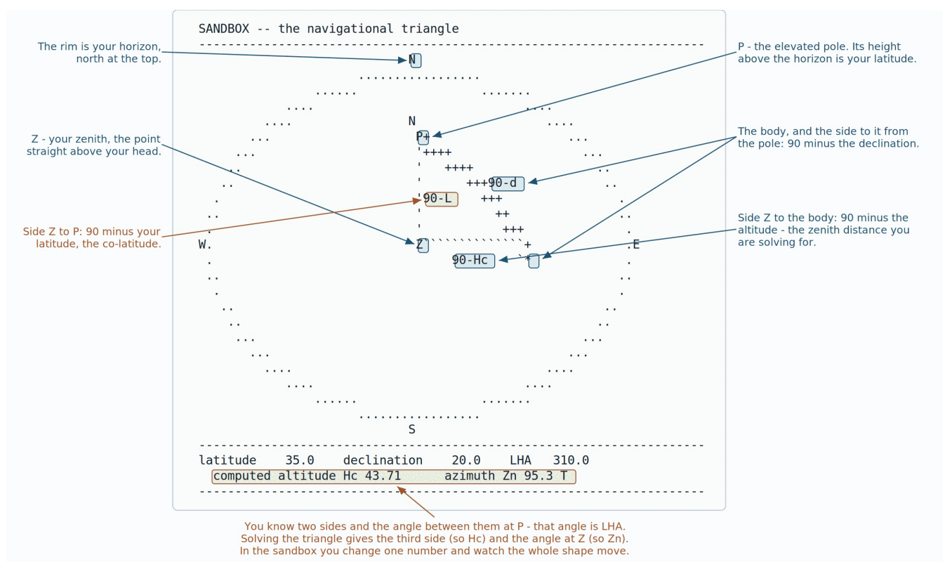
Figure 8 — the sandbox. This is the same triangle the reduction solves for every sight you take.
