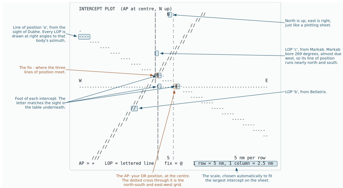
Figure 4 — the intercept plot. It is a plotting sheet drawn in characters: your DR at the centre, one lettered line for each sight, and the fix where they cross. The letters match the summary table printed underneath it.
