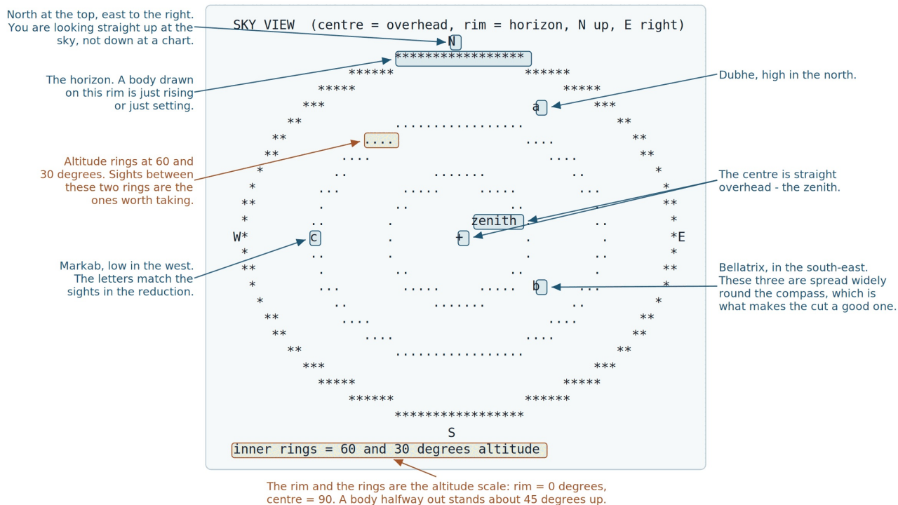
Figure 2 — the sky view from celnav plan , and the same diagram after a reduction. It is a picture of the sky above you, not a chart: the point straight overhead is at the centre and the horizon is the outer rim, so a body near the rim is low down and one near the centre is nearly overhead.
