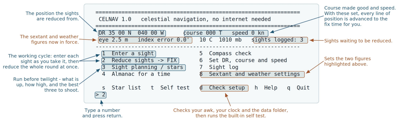
Figure 1 — the main menu. The two status lines at the top always show what the next reduction will be based on, so you can see at a glance whether the DR, the run and the sextant settings are the ones you meant.
