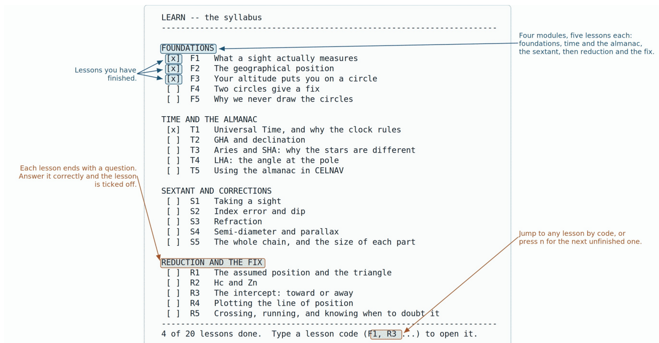
Figure 6 — the syllabus. Type a code to open any lesson, or press n for the next one you have not finished.
