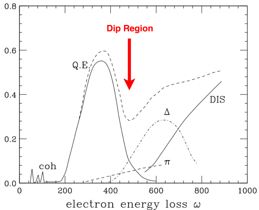
Quasi-Elastic Electron-Nucleus Scattering
