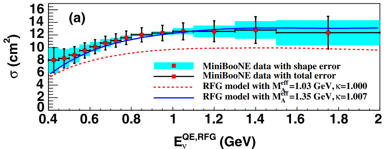
Quasi-Elastic(-Like) Neutrino-Nucleus Cross-Section
