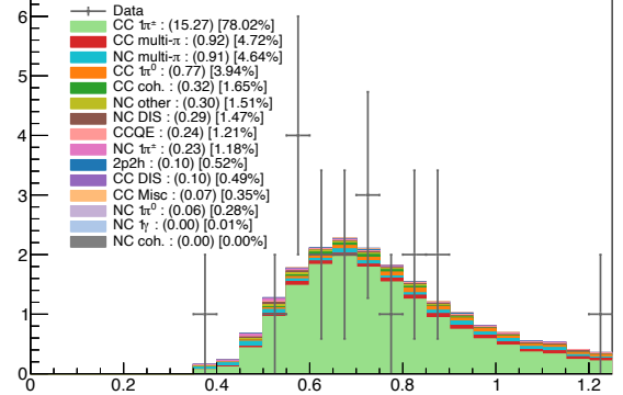
FHC \nu_e CC1 \pi^+ Sample – MC and Data
