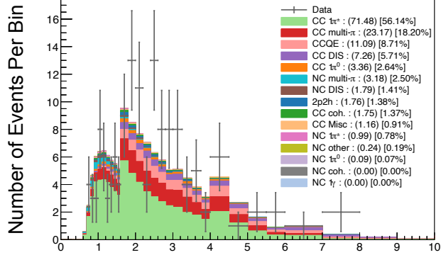
FHC \nu_\mu CC1 \pi^+ Sample – MC and Data
