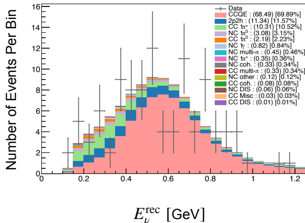
FHC 1e-Ring Sample – MC and Data
