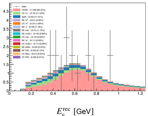
RHC 1e-Ring Sample – MC and Data
