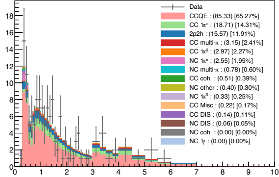
RHC 1\mu -Ring Sample – MC and Data
