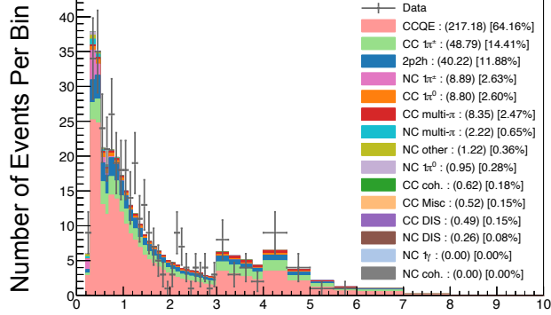
FHC 1\mu -Ring Sample – MC and Data
