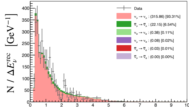
FHC 1\mu -Ring Sample – MC and Data
