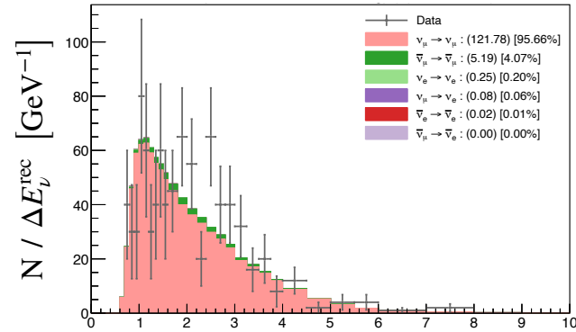
FHC \nu_\mu \text{CC}1\pi^+ Sample – MC and Data
