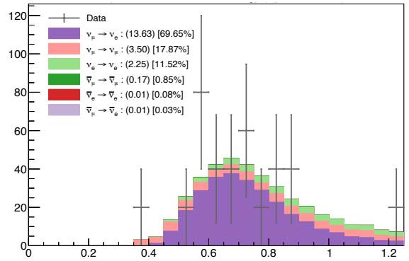
FHC \nu_e \text{CC}1\pi^+ Sample – MC and Data
