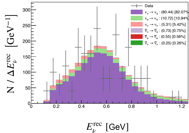
FHC 1e-Ring Sample – MC and Data
