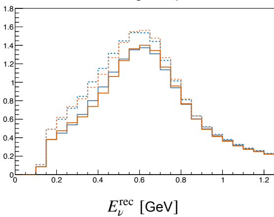
RHC 1e-Ring Sample – MC
