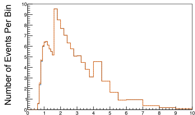
FHC \nu_\mu \text{CC}1\pi^+ Sample – MC
