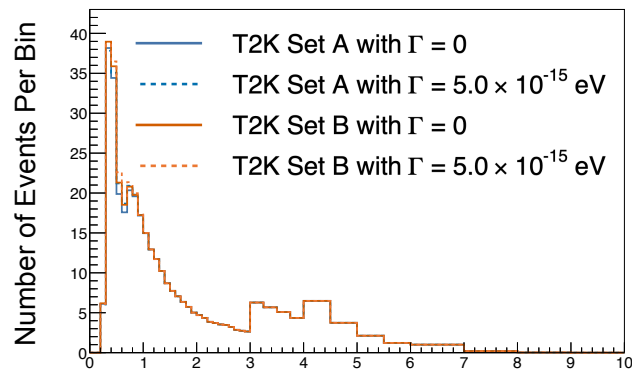
FHC 1\mu -Ring Sample – MC
