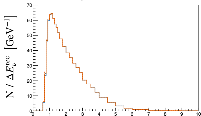
FHC \nu_\mu \text{CC}1\pi^+ Sample – MC
