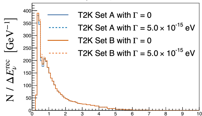
FHC 1\mu -Ring Sample – MC
