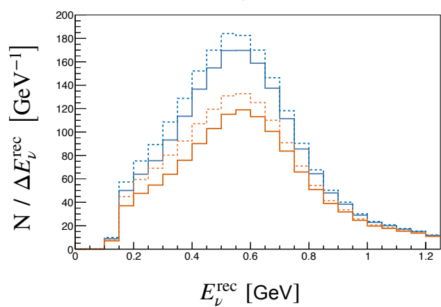
FHC 1e-Ring Sample – MC
