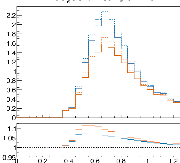
FHC \nu_e \text{CC}1\pi^+ Sample – MC
