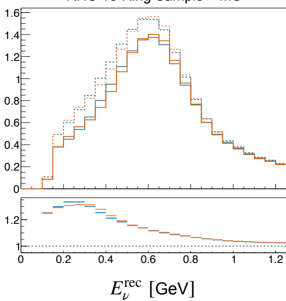
RHC 1e -Ring Sample – MC
