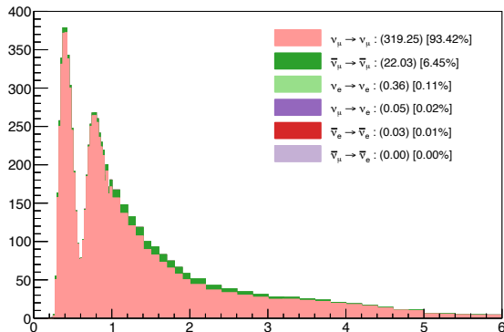
FHC 1 \mu -Ring Sample – True \nu Energy
