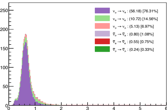
FHC 1e-Ring Sample – True \nu Energy
