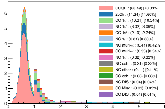
RHC 1e-Ring Sample – True \nu Energy
