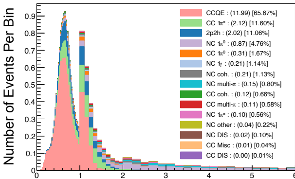
FHC 1e-Ring Sample – True \nu Energy
