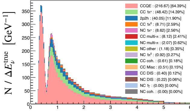
FHC 1\mu -Ring Sample – True \nu Energy
