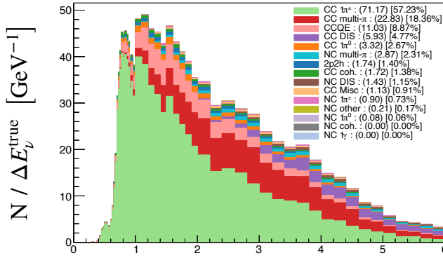
FHC \nu_\mu CC1 \pi^+ Sample – True \nu Energy
