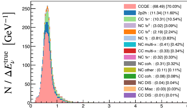
FHC 1e-Ring Sample – True \nu Energy
