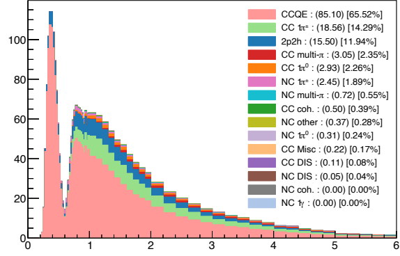
RHC 1\mu -Ring Sample – True \nu Energy
