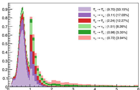
RHC 1e-Ring Sample – True \nu Energy
