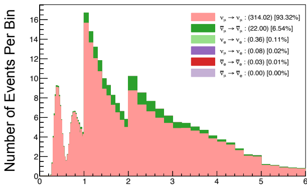
FHC 1\mu -Ring Sample – True \nu Energy
