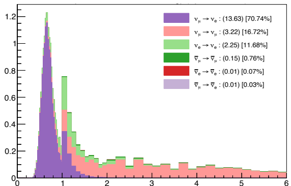
FHC \nu_e CC 1\pi^+ Sample – True \nu Energy
