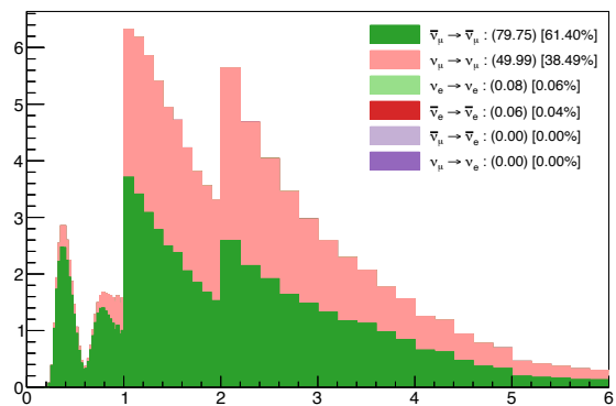
RHC 1\mu -Ring Sample – True \nu Energy
