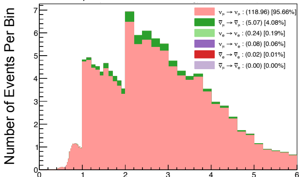
FHC \nu_\mu CC 1\pi^+ Sample – True \nu Energy
