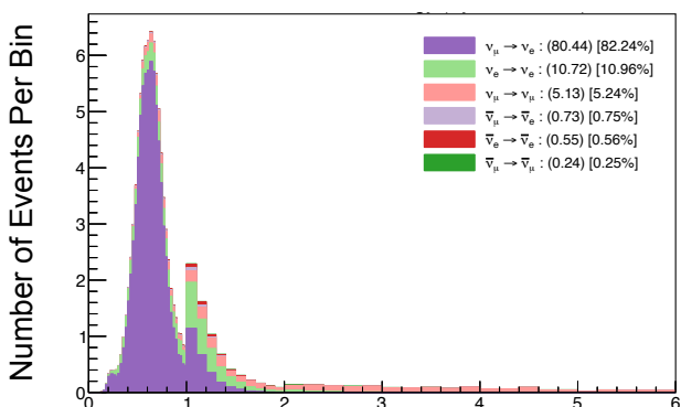
FHC 1e-Ring Sample – True \nu Energy
