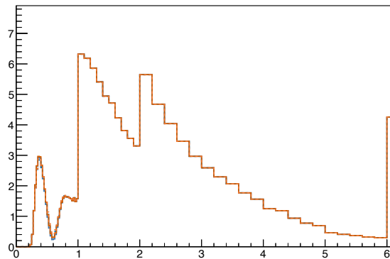
RHC 1\mu -Ring Sample – MC
