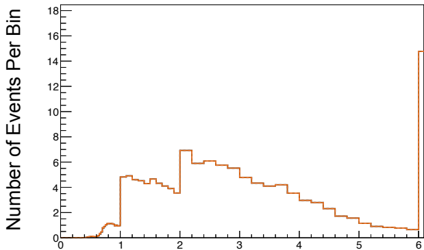
FHC \nu_\mu \text{CC}1\pi^+ Sample – MC
