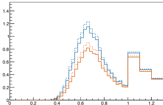
FHC \nu_e \text{CC}1\pi^+ Sample – MC
