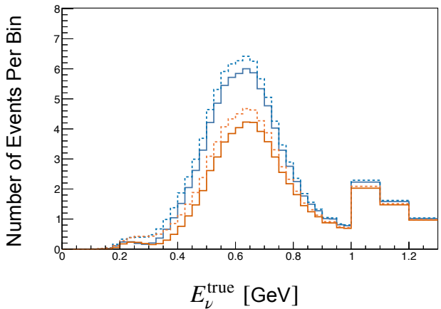
FHC 1e-Ring Sample – MC
