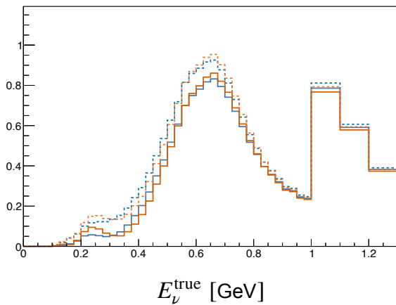
RHC 1e-Ring Sample – MC
