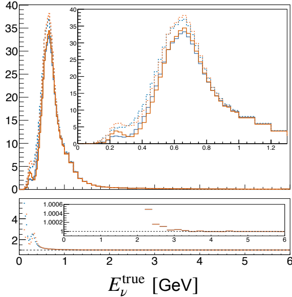
RHC 1e -Ring Sample – MC
