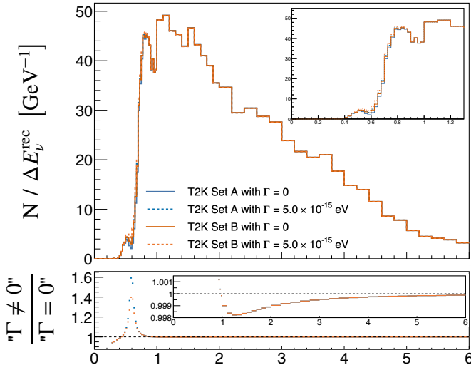
FHC \nu_\mu \text{CC}1\pi^+ Sample – MC
