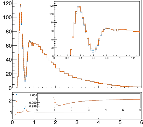
RHC 1\mu -Ring Sample – MC
