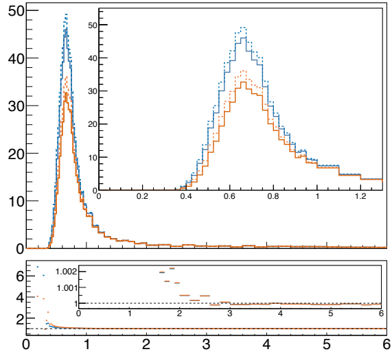
FHC \nu_e \text{CC}1\pi^+ Sample – MC
