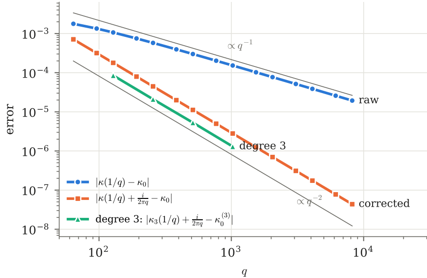
FIGURE 1. Convergence of \kappa(1/q) to \kappa_0 (degree two) and of \kappa_3(1/q) to \kappa_0^{(3)} (degree three, Section 7). The raw error decays like q^{-1} ; after the universal correction -i/(2\pi q) it decays like q^{-2} . Grey lines are slope guides.
