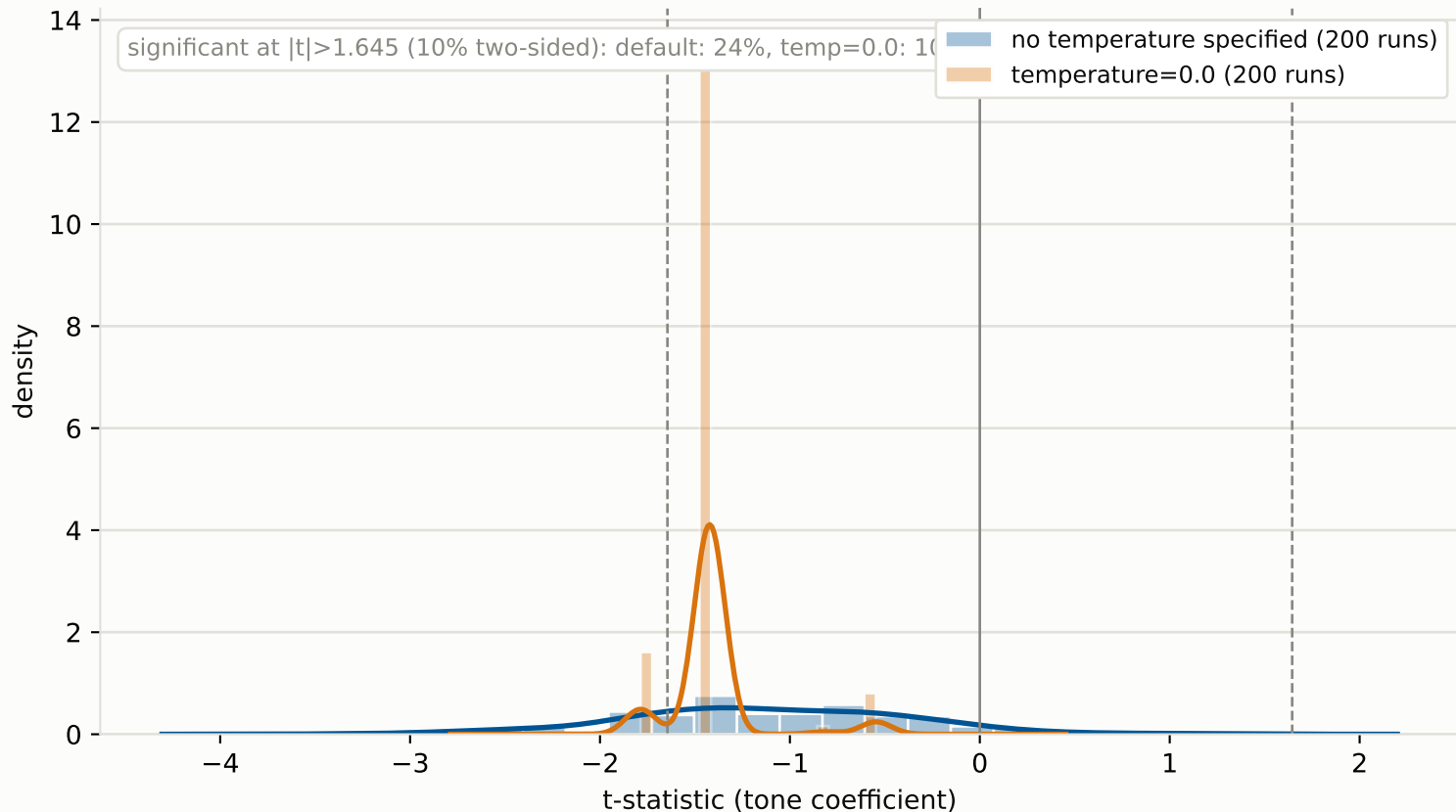
deepseek-v4-pro: distribution of t-statistics, both conditions (2025-01-01 to 2026-01-01 return ~ digitized sentiment)
