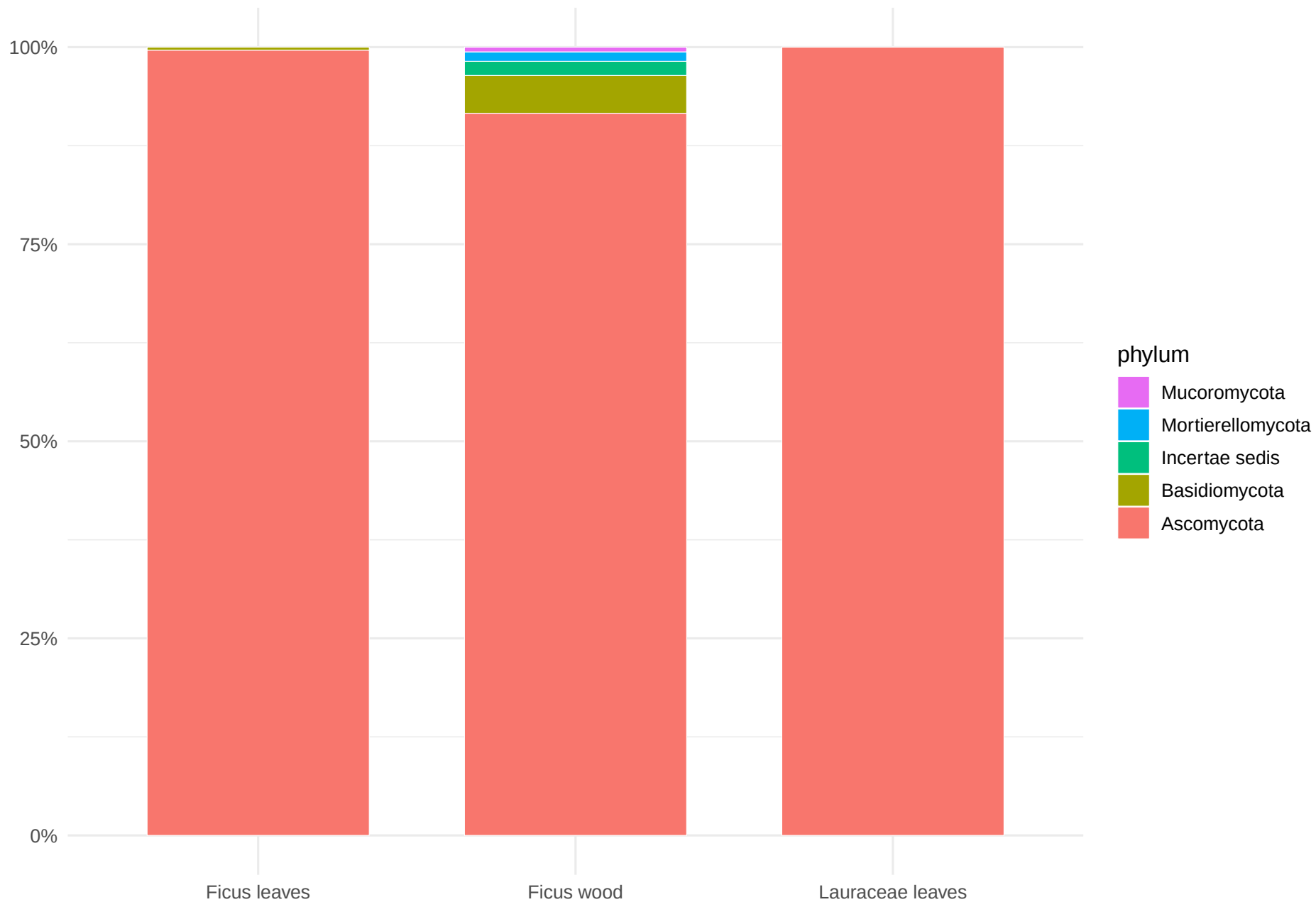
Relative abundance by phylum
