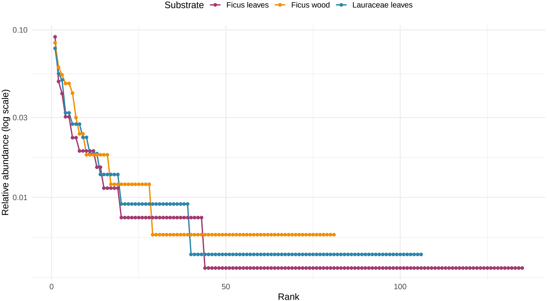
Rank–abundance curve — its_taxon
