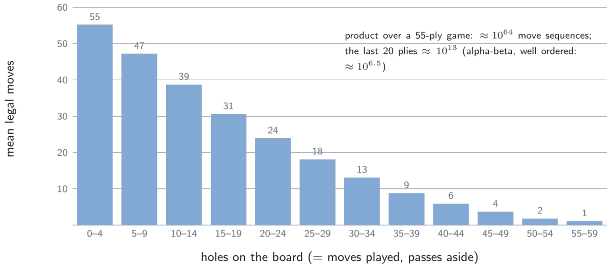
Figure 22: Mean number of legal moves as a function of the number of holes, measured on self-play positions.
