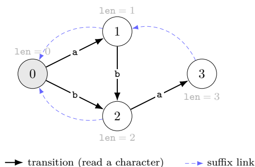
Suffix automaton of aba
