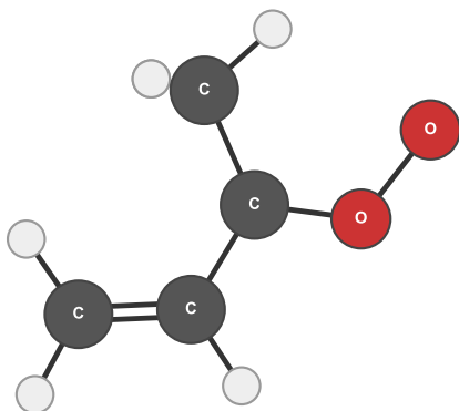
trans syn-trans
