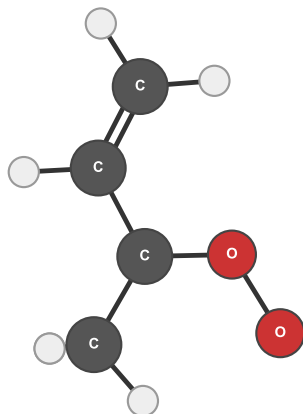
cis syn-cis
