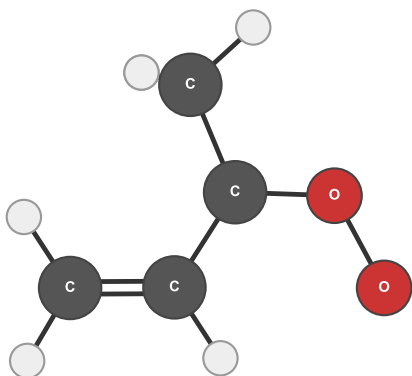
anti-trans
