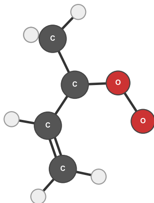
anti-cis
