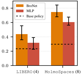
Critic architecture
