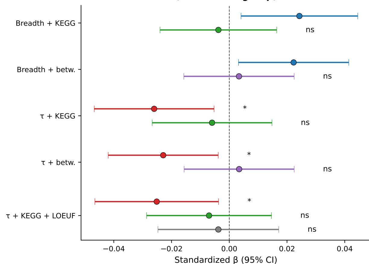
C. PBS-1 African (S. Asian outgroup) — coefficients
