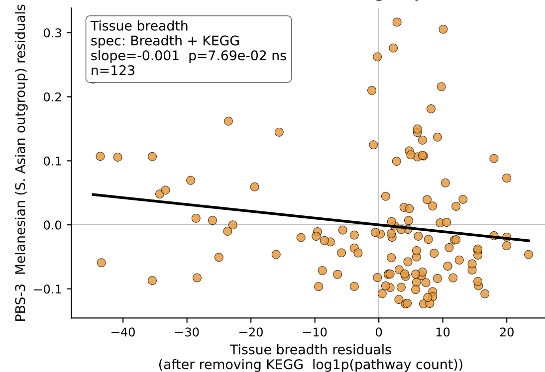
B. PBS-3 Melanesian (S. Asian outgroup) — added-variable
