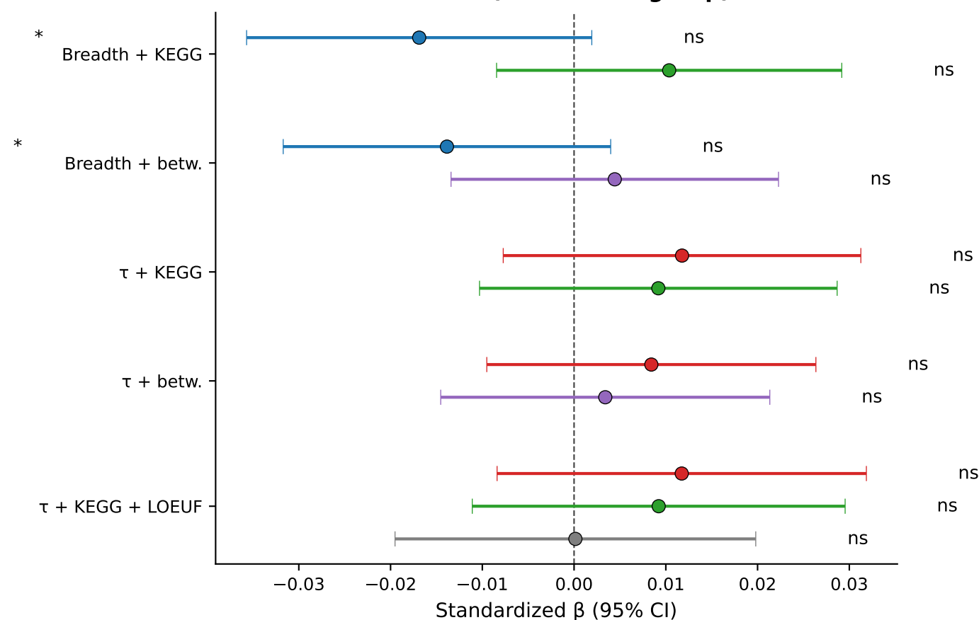
D. PBS-3 Melanesian (S. Asian outgroup) — coefficients
