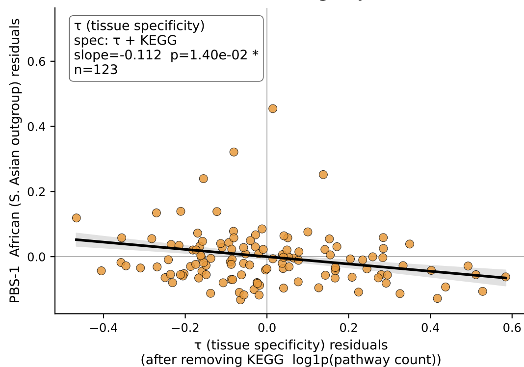
A. PBS-1 African (S. Asian outgroup) — added-variable
