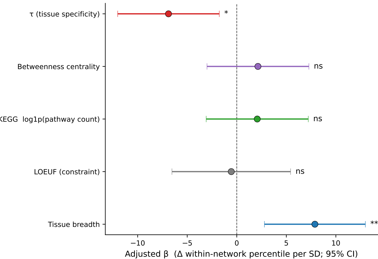
EUR — European (Afr-Mel reference)
