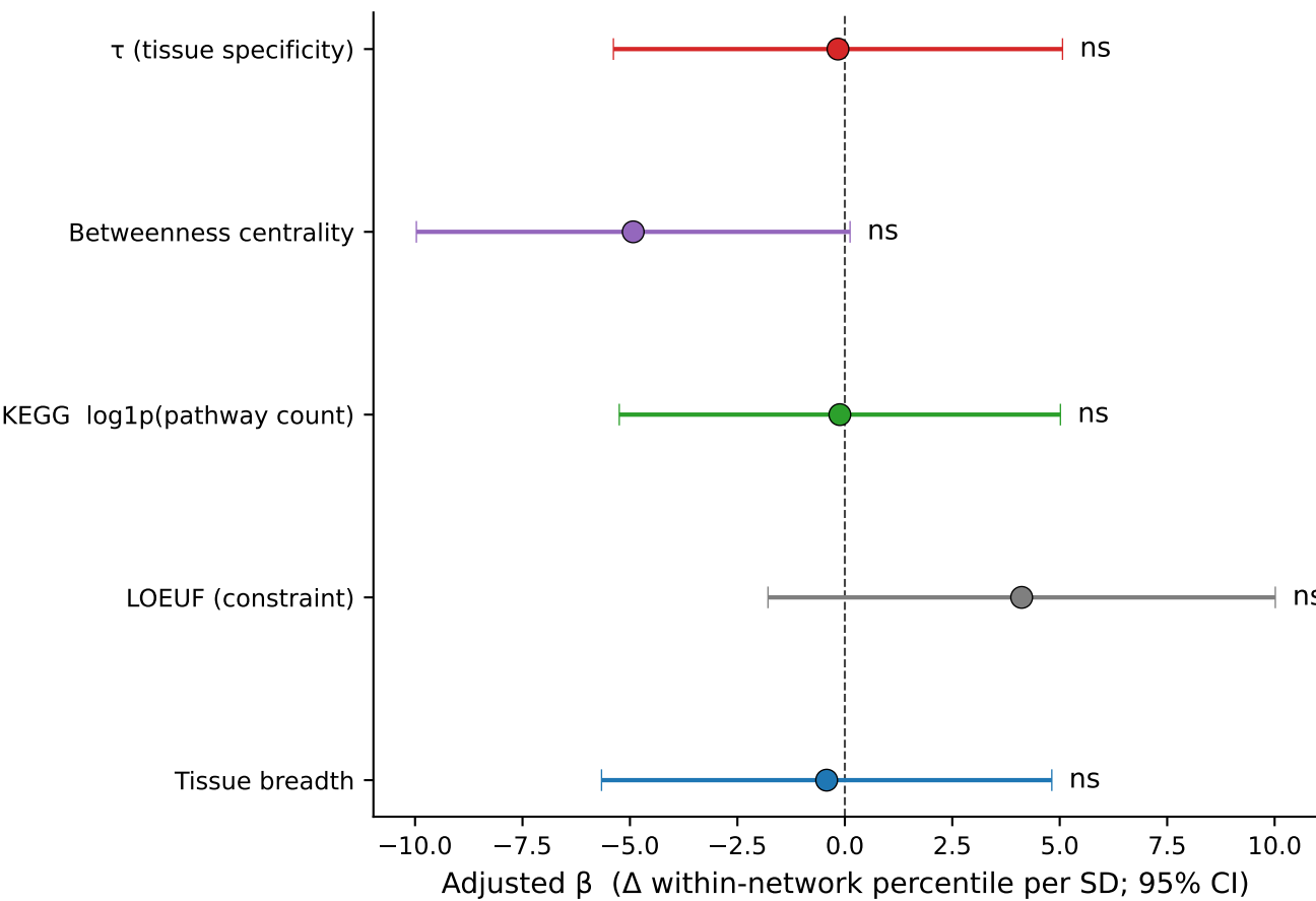
SAS — South Asian (Afr-Mel reference)
