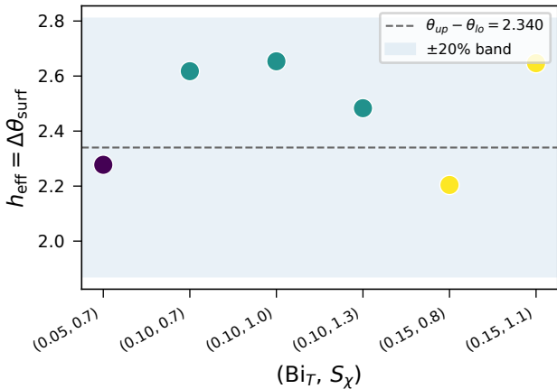
(b) Amplitude collapse
