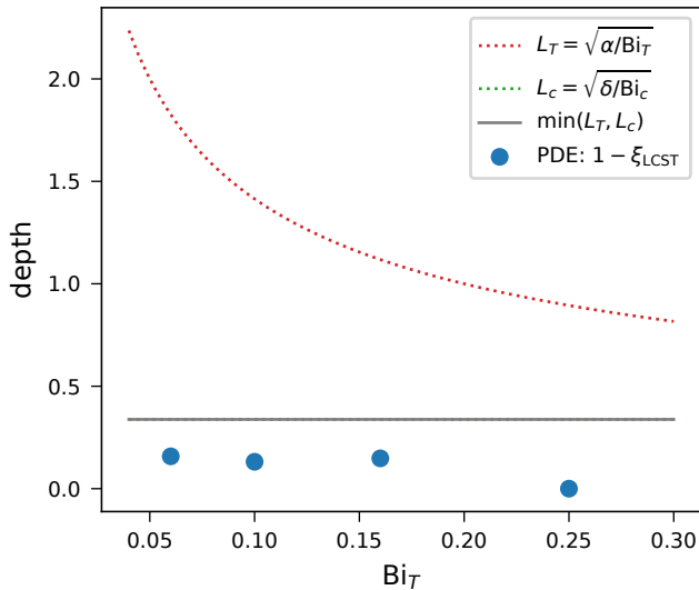
(b) \text{Bi}_T slice ( m_{\text{act}} = m_{\text{diff}} = 4 )
