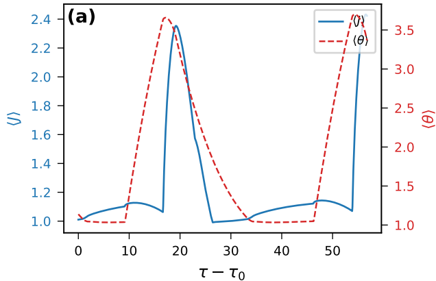
Regime II: S_\chi = 1.0 , Da = 9.5 (thermal breathing)
