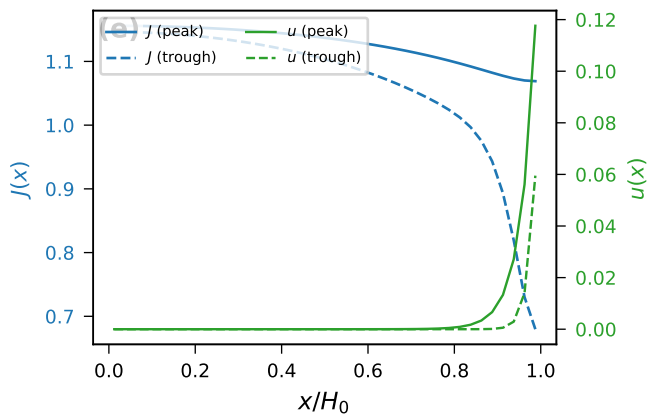
Spatial profiles — Regime II
