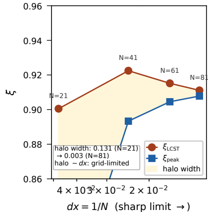
(c) N convergence
