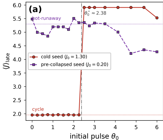
C-cell IC-induced hysteresis: \text{Bi}_T = 0.059 , S_\chi = 1.80 , u_0 = 0.50
