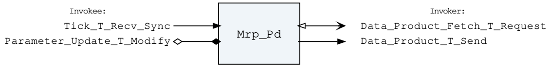
Figure 1: Mrp Pd component diagram.
