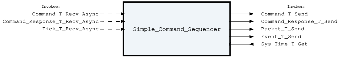
Figure 1: Simple Command Sequencer component diagram.
