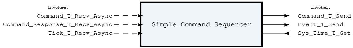
Figure 1: Simple Command Sequencer component diagram.
