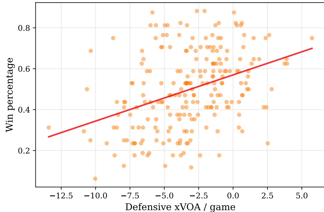
Defense vs Win% r = 0.376 , R^2 = 14.2\%
