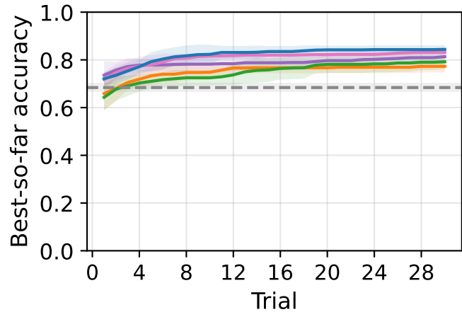
HotpotQA
