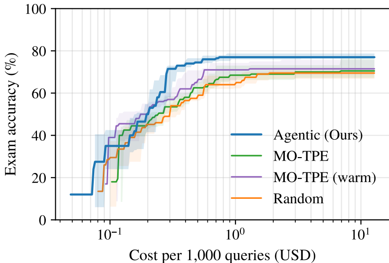
Cost vs exam accuracy on UniDoc (healthcare)
