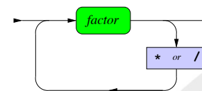
term
