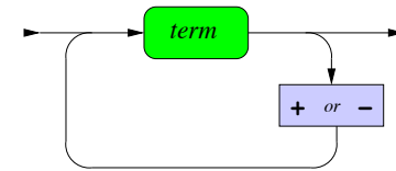
expression
