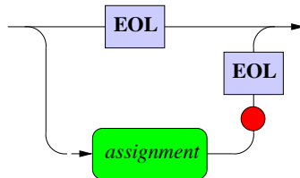
statement
