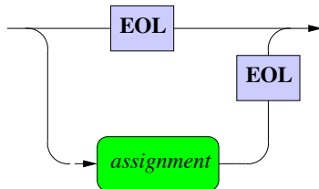
statement
