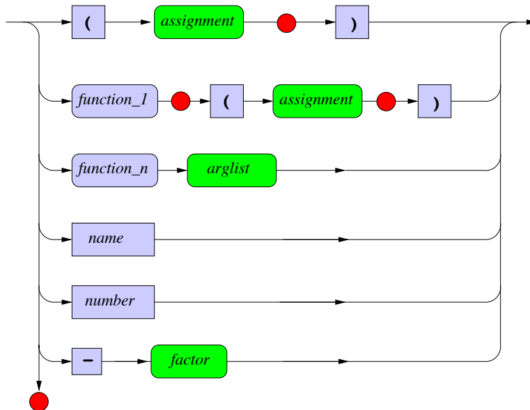
factor
