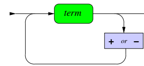
expression
