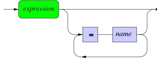
assignment
