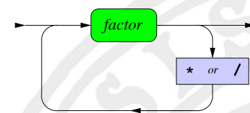
term
