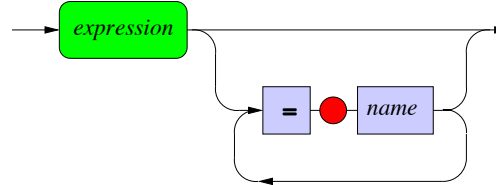
assignment
