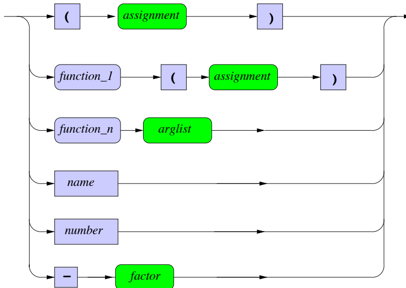
factor
