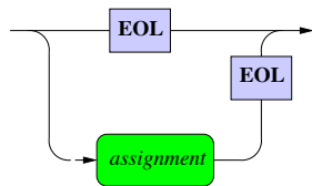
statement
