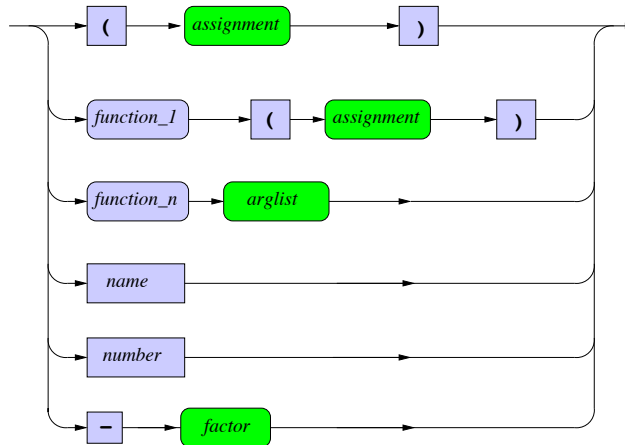
factor
