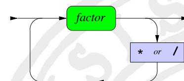
term
