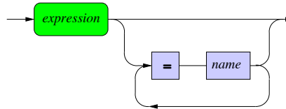
assignment
