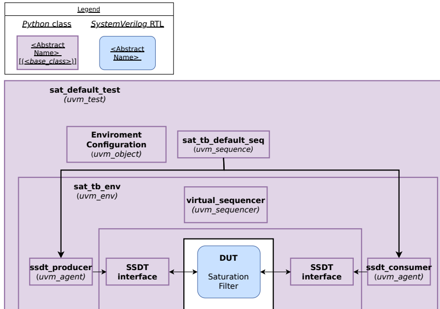
Fig. 1: Testbench overview with producer and consumer UVC agents.
