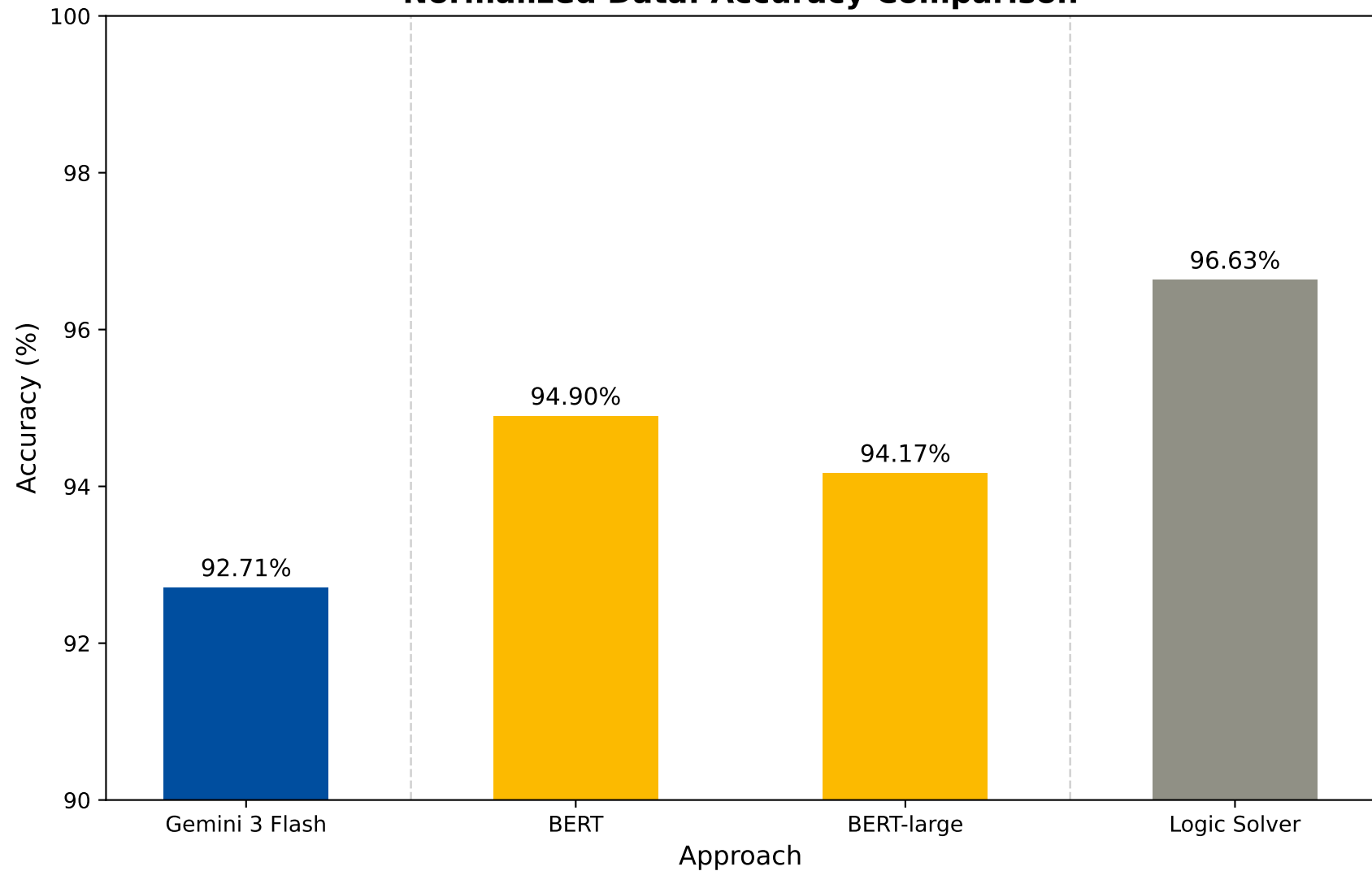
Normalized Data: Accuracy Comparison
