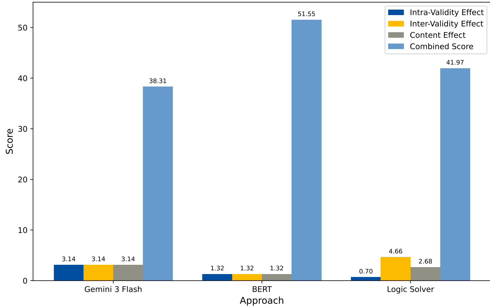
Normalized Data: Content Effect and Combined Score
