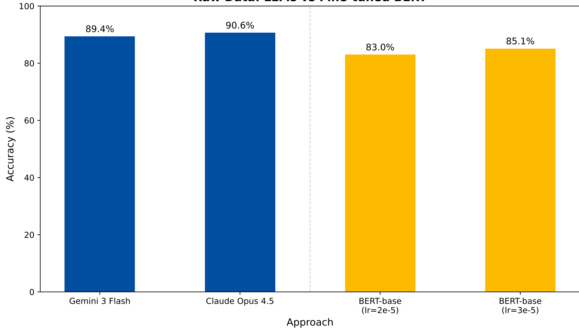
Raw Data: LLMs vs Fine-tuned BERT
