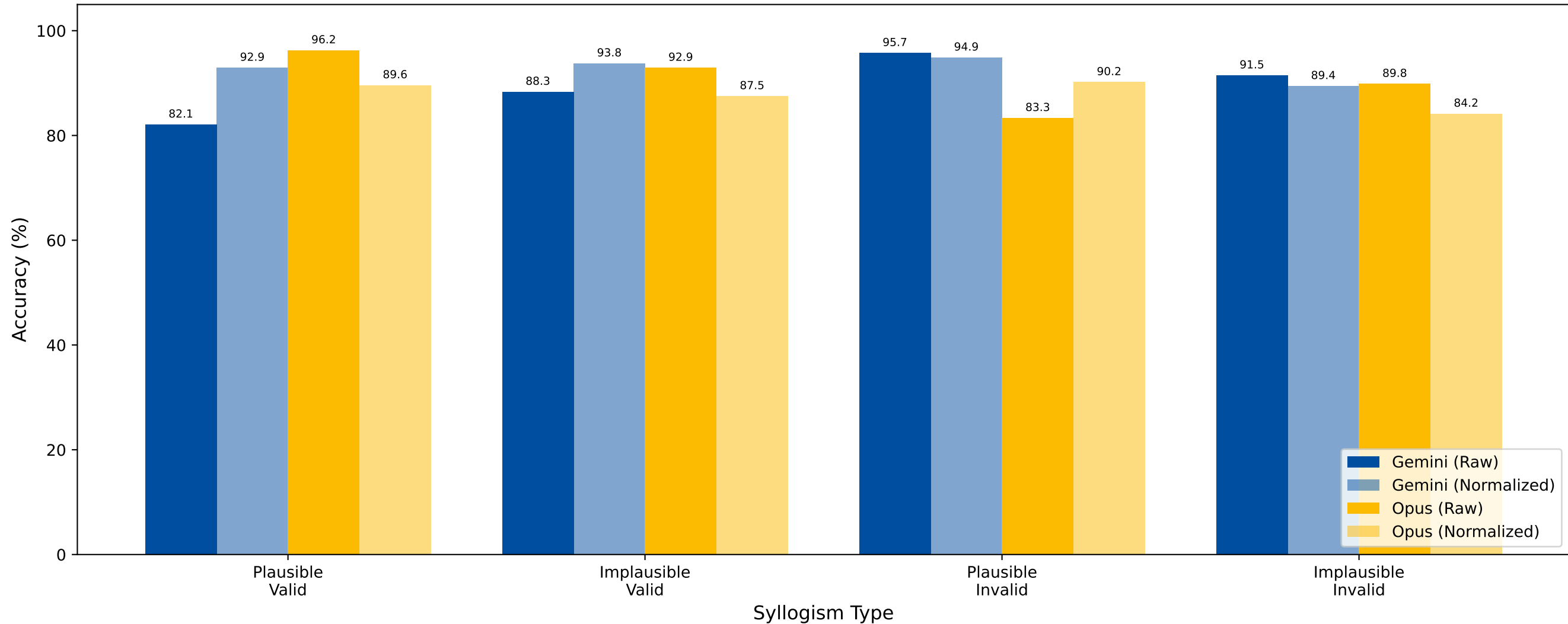
Accuracy by Syllogism Type: Gemini vs Claude Opus
