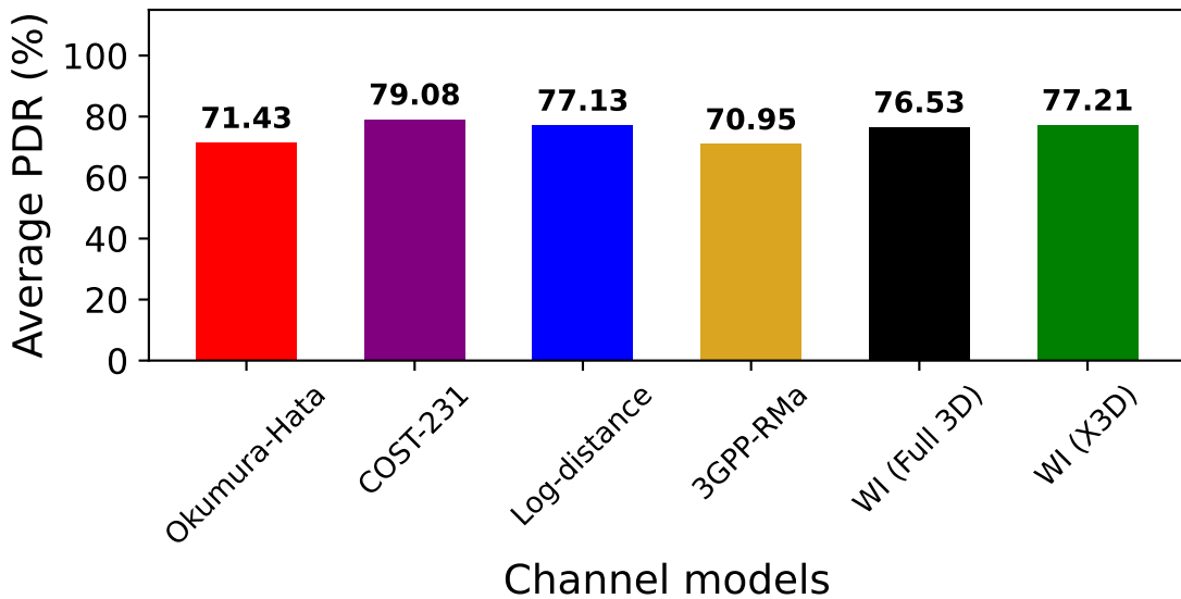
Average PDR across all GWs in Forest ( \gamma = 0.7 )
