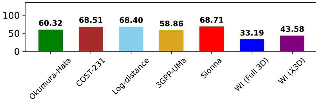
Average PDR across all GWs in grid 2 and St. Canyon ( \rho = -90 )
