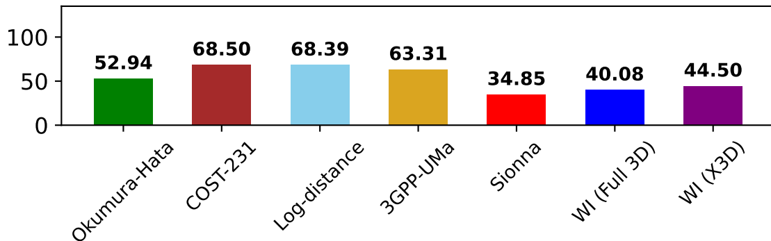
Average PDR across all GWs in grid 1 and Etoile ( \rho = -90 )
