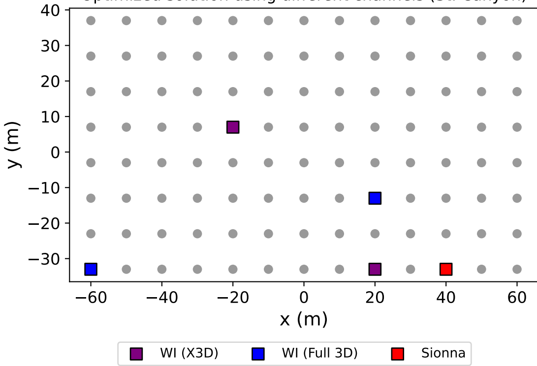
Optimized solution using different channels (St. Canyon)
