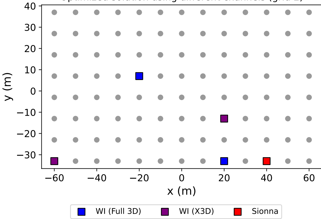
Optimized solution using different channels (grid 2)
