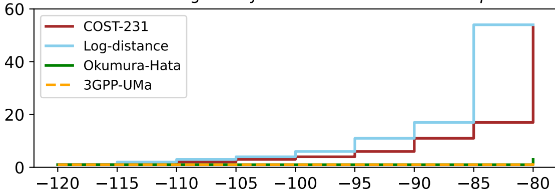
Number of gateways across different values of \rho
